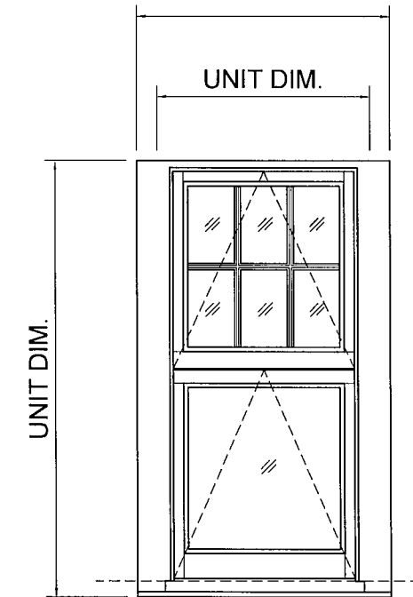
EXTERIOR ELEVATION OF SERIES 5000 IN-LINE FOLD-UP IN WINDOW UNIT AT COUNTER
